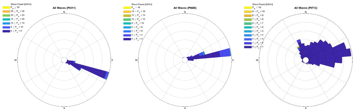
Figure B8: Wave rose for discrete points around St. Croix: Northeast (Pt. 311), Southeast (Pt. 686), and Northeast (Pt. 713)
