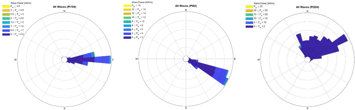
Figure B2: Wave rose for discrete points around St. John: Northeast (Pt. 194), Southeast (Pt. 82), and Northeast (Pt. 204).
