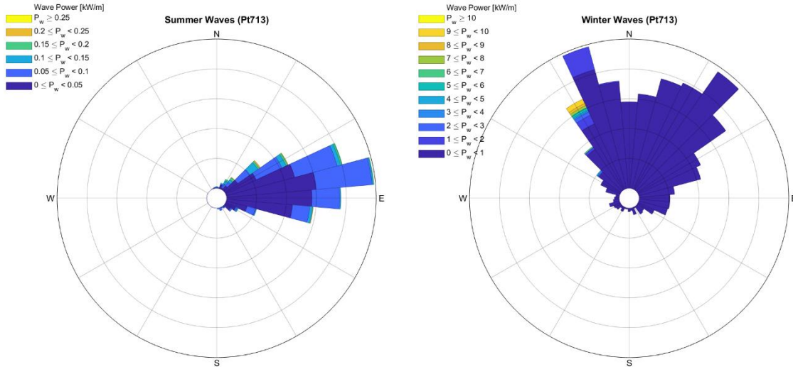
Figure B9: Summer and winter wave climate northeast of St. Croix
