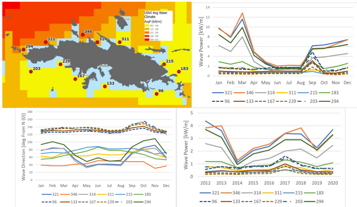
Figure B4: Wave climate around St. Thomas and monthly averaged time series of wave power (upper right) and wave direction (lower left), and yearly averaged time series of wave power (lower right).
