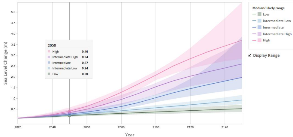
Figure 11: Projections of sea-level rise values on St. Croix. Screenshot from NASA online tool 26
