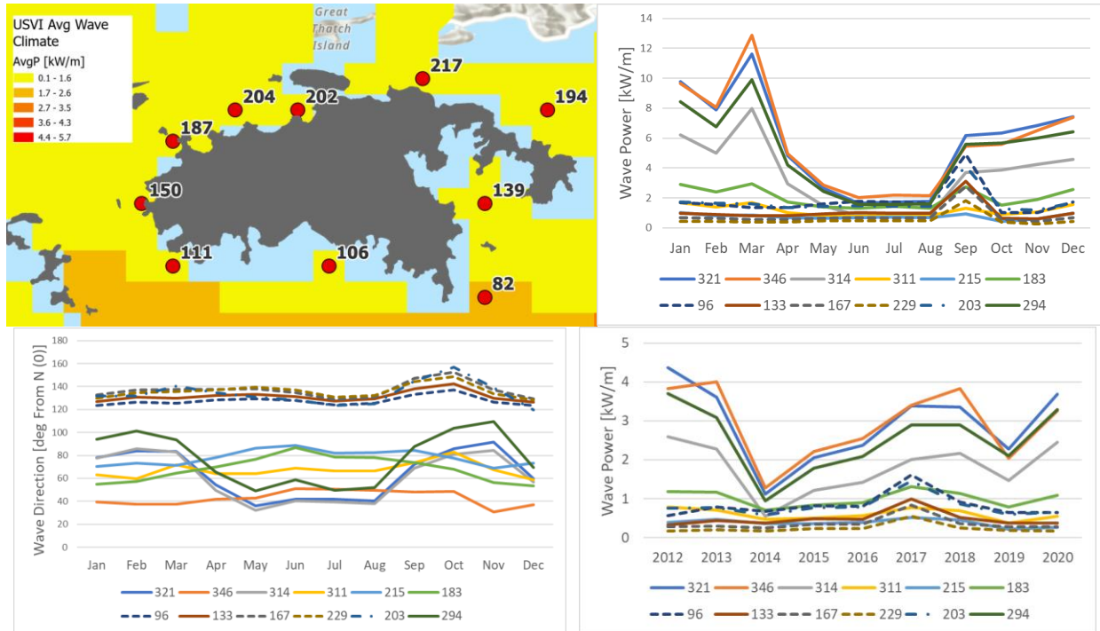
Figure B1: Wave climate around St. John and monthly averaged time series of wave power (upper right) and wave direction (lower left), and yearly averaged time series of wave power (lower right).
