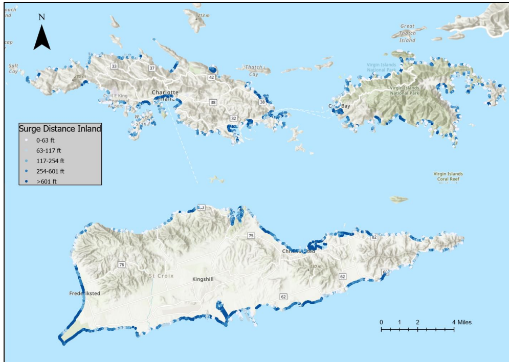
Figure 16: Storm surge inundation distance from the coast as computed by the SLOSH model 9
