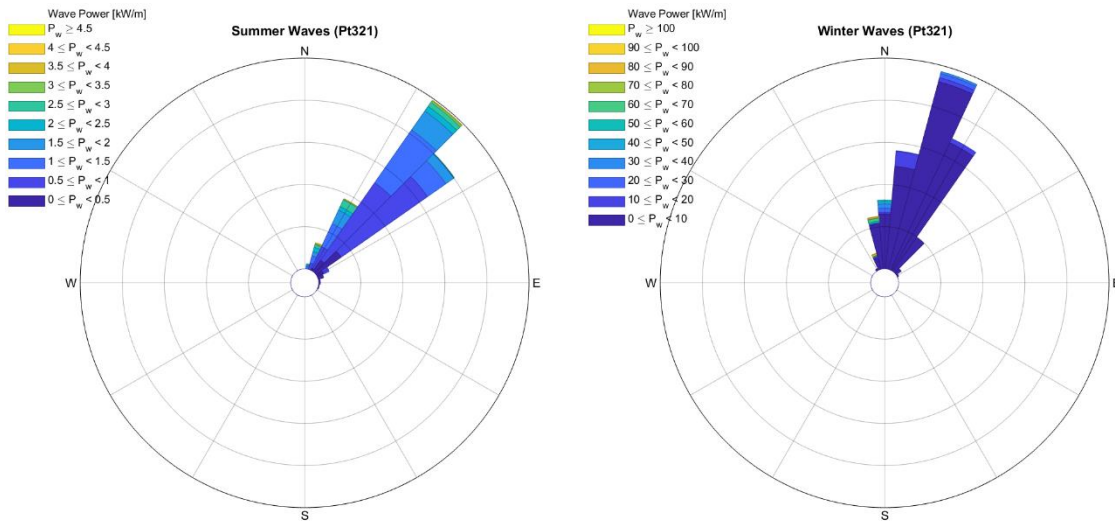
Figure B6: Summer and winter wave climate northeast of St. Thomas
