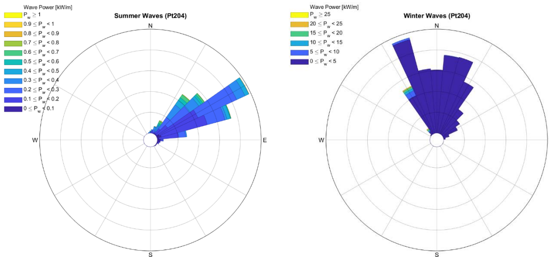
Figure B2: Wave rose for discrete points around St. John: Northeast (Pt. 194), Southeast (Pt. 82), and Northeast (Pt. 204).
