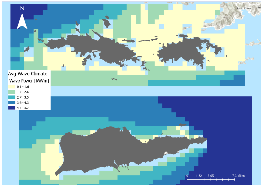
Figure 18: Wave power climate around the USVI
