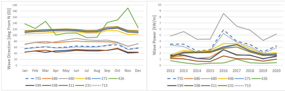
Figure B7: Wave climate around St. Croix and monthly averaged time series of wave power (upper right) and wave direction (lower left), and yearly averaged time series of wave power (lower right).
