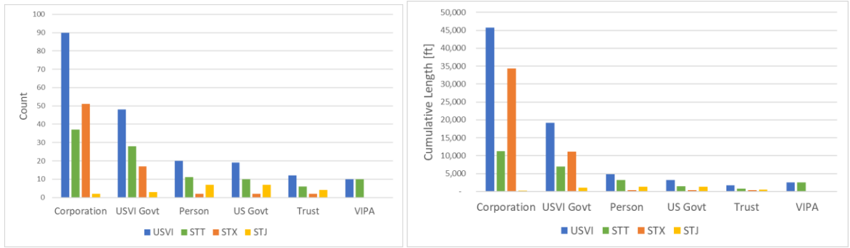
Figure 8: Amount and length of coastal armoring by different types of owners
